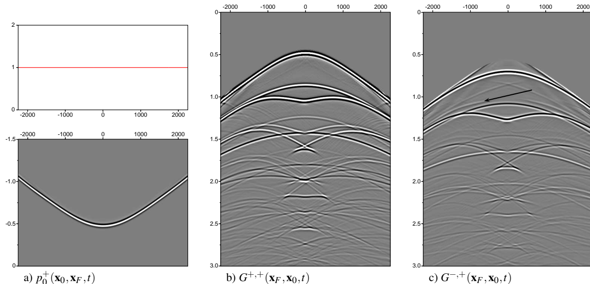
Figure 5: Up- and downgoing wavefields after 15 iterations with an amplitude error in p_0^+ . The amplitude along the wavefield is flat for all offsets as shown in the amplitude plot in (a). In the upgoing Green's function (c) only a few ghosts events, with a low amplitude and indicated with an arrow, are introduced.
