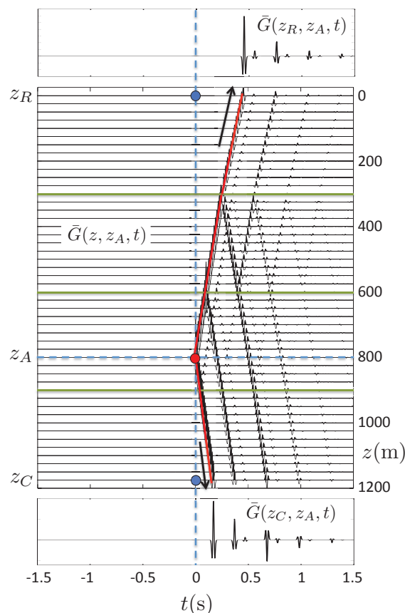
Figure 2: The Green's function \bar{G}(z, z_A, t) in a horizontally layered medium. In equation (4) we need an auxiliary function \Gamma(z, t) which, at z_C = 1175 m, cancels this Green's function.
