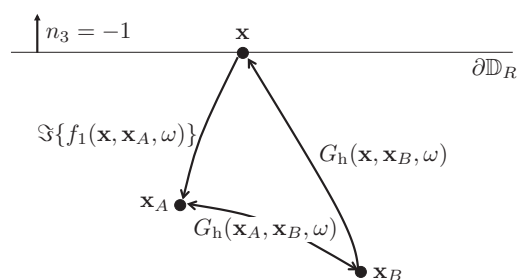
Figure 7: Visualisation of the single-sided homogeneous Green's function representation (equation 7). Similar as in Figure 1, the rays represent the full responses between the source and receiver points, including multiple scattering.
