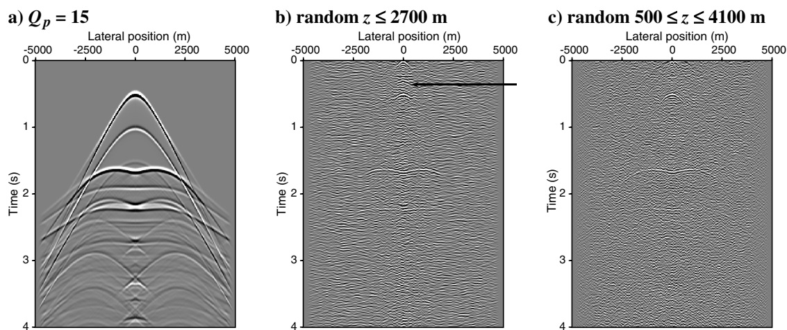
Figure 10. Reflection results in viscoacoustic media with constant quality factor Q_p = 15 ; (a) the directly modeled result; (b) and (c) show the SI results for two source distributions as indicated in the text below the panels.
